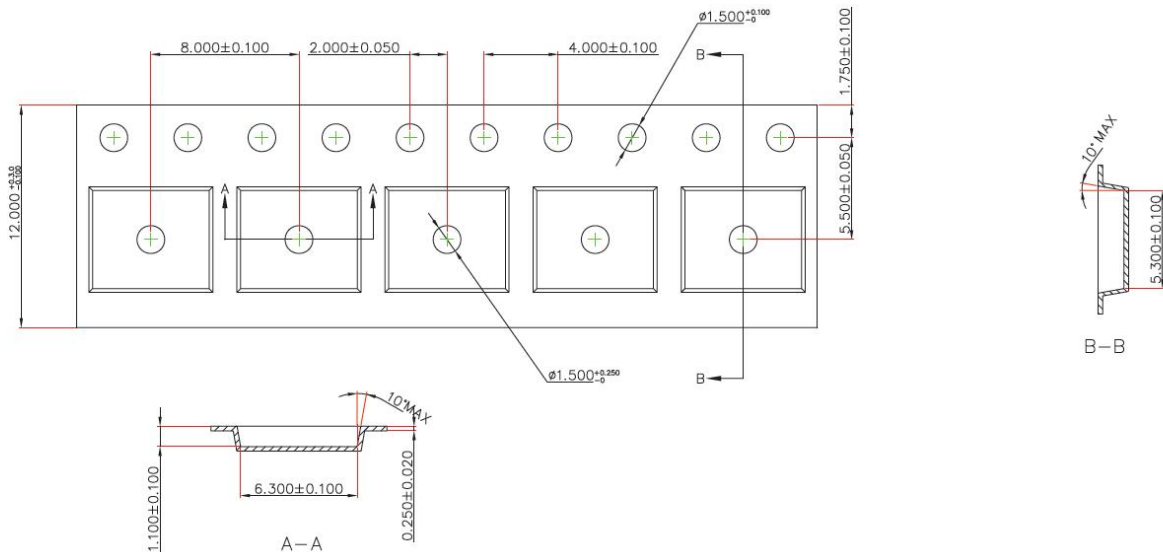
Fig 3. Carrier tape dimensions
